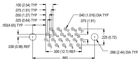
21 Socket MWDM-21SCBS
