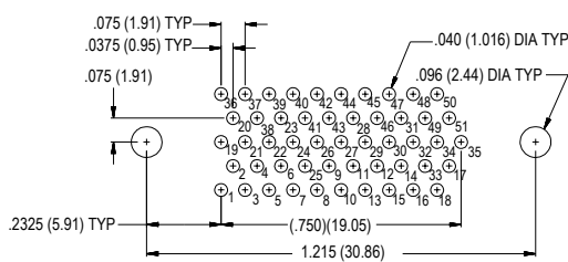
51 Socket MWDM-51SCBS
