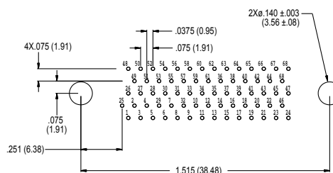
69 Socket MWDM-69SCBS
