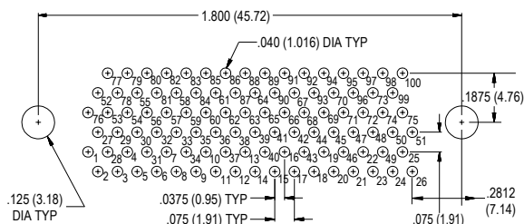
100 Socket MWDM-100SCBS
