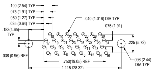
31 Socket MWDM-31SCBS
