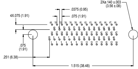
69 Socket MWDM-69SCBS
