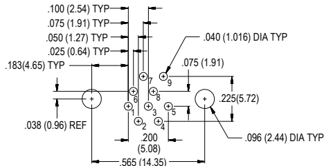
9 Socket MWDM-9SCBS
