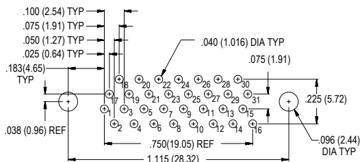
31 Socket MWDM-31SCBS
