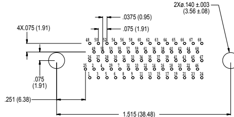
69 Socket MWDM-69SCBS
