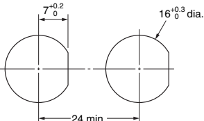
Panel Cutouts
