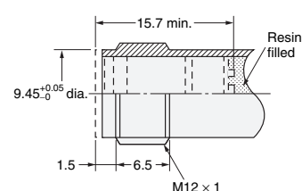
Mounted Dimensions
