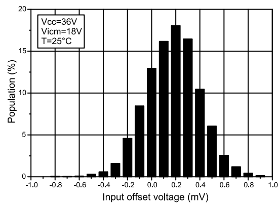
Figure 4: Input offset voltage distribution at V_{CC} = 36\text{ V}
