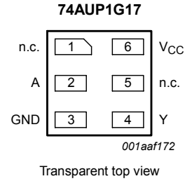
Figure 5. Pin configuration SOT886, SOT891, SOT1115 and SOT1202
