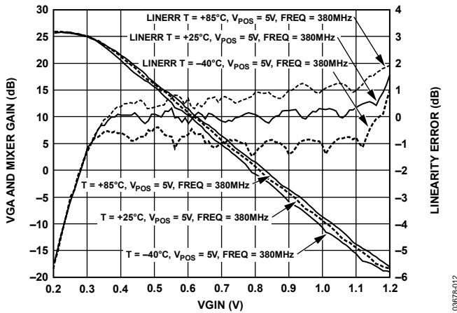
Figure 12. Mixer Gain and Linearity Error vs. VGIN, V_{POS} = 5V , F_{IF} = 380MHz , F_{BB} = 1MHz , Temperature = -40^{\circ}C , +25^{\circ}C , +85^{\circ}C
