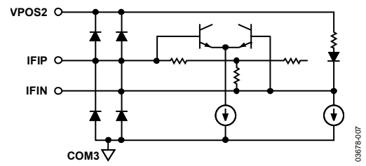
Figure 7. Circuit E
