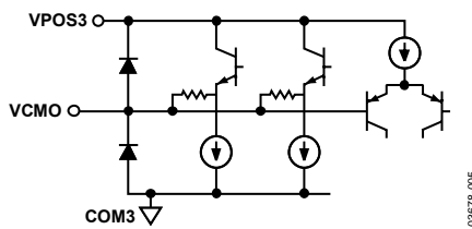
Figure 5. Circuit C
