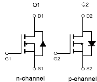
n-channel p-channel Equivalent Circuit
