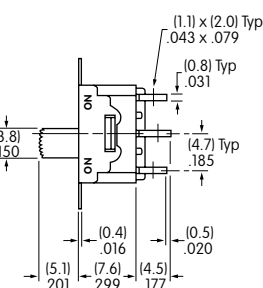
Actuator in LEFT Position
