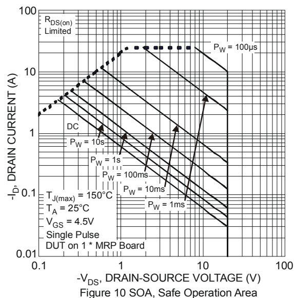
Figure 10 SOA, Safe Operation Area
