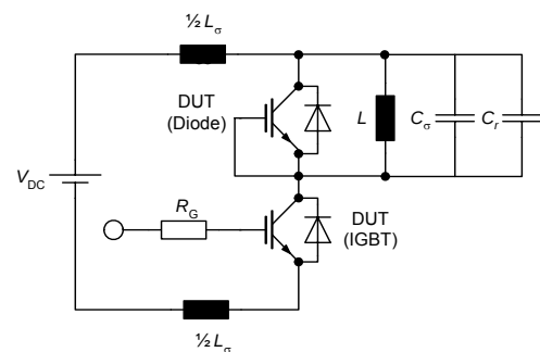
Figure E. Dynamic test circuit Leakage inductance L_\sigma = 180\text{nH} , Stray capacitor C_o = 40\text{pF} , Relief capacitor C_r = 4\text{nF} (only for ZVT switching)
