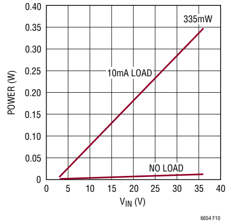
Figure 10. Typical Power Dissipation of the LT6654
