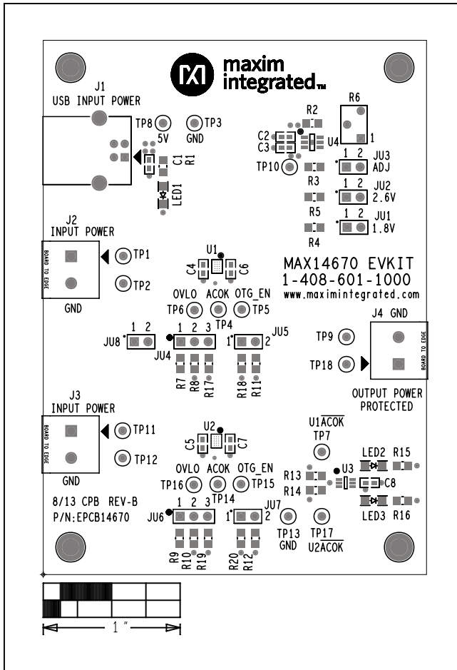
Figure 2. MAX14670 EV Kit Component Placement Guide—Component Side
