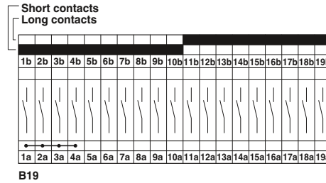
6 (10) mm 2 , 30 A, test terminal strip, for wall mounting, VDE coded type B19
