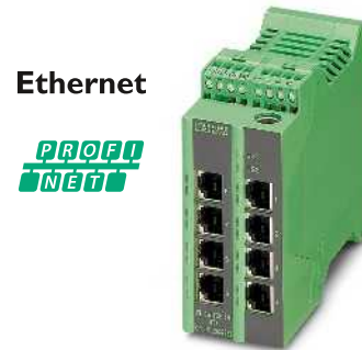
8 RJ45 ports
