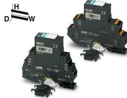
2 double conductors (loops), floating, 9/10 connection grounded directly
