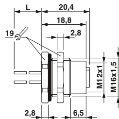
Dimensions: socket
