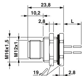
Dimensions: plug
