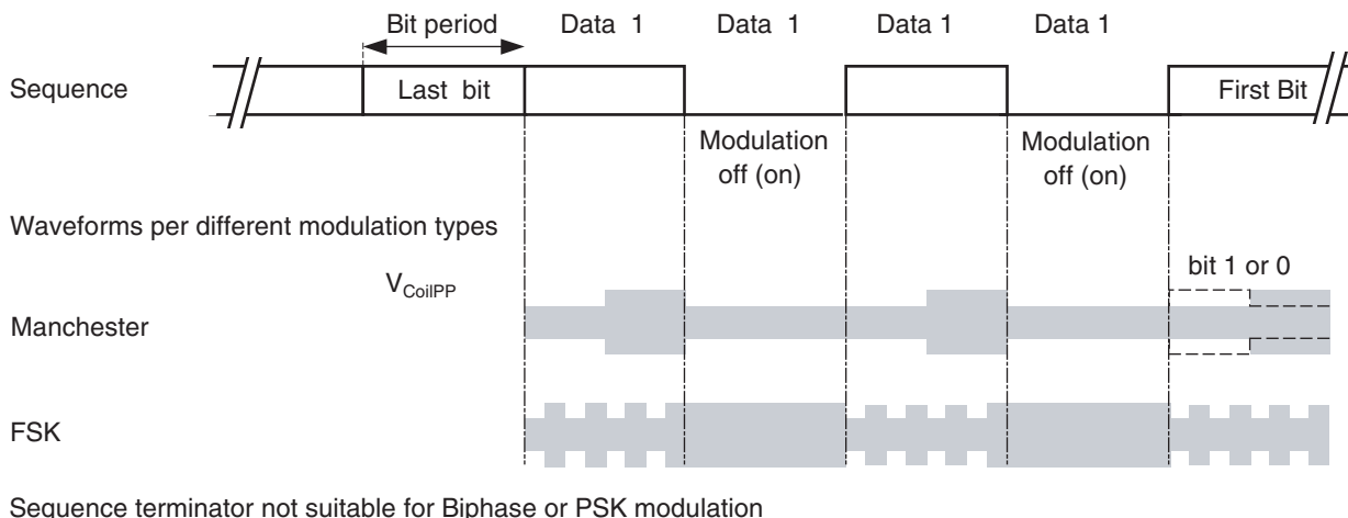
Figure 4-3. e5550-compatible Sequence Terminator Waveforms
