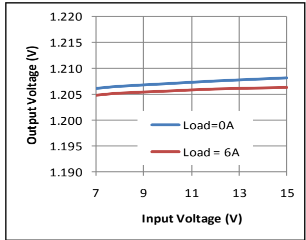
Figure 13. Line Regulation
