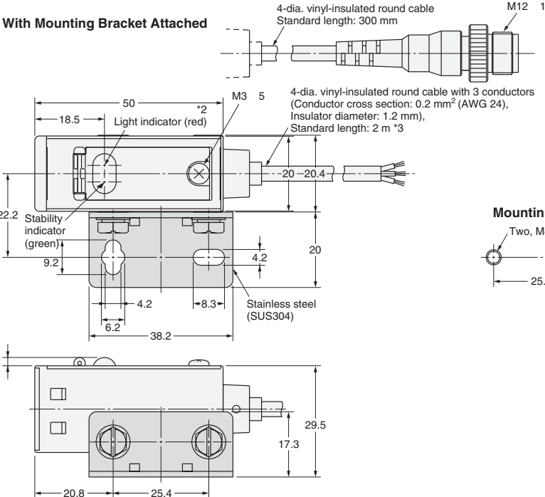
Pre-wired Connector (-M1J)
