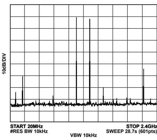
Figure 28. Single-Tone Spectrum in Mix Mode at f_{OUT} = 1.31\text{ GHz} , f_{DAC} = 2.4\text{ GSPS}
