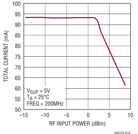
Total Current vs RF Input Power
