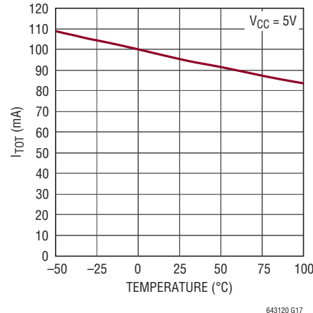
Total Current ( I_{TOT} ) vs Temperature
