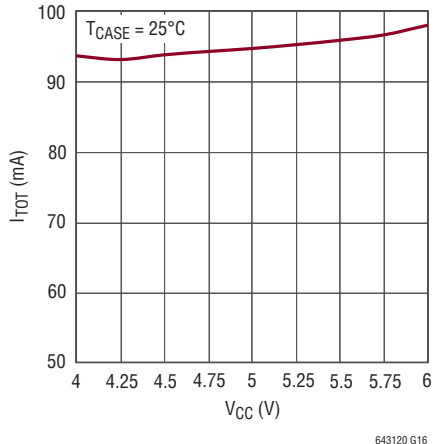
Total Current ( I_{TOT} ) vs V_{CC}
