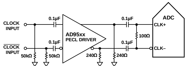
Figure 51. Differential PECL Sample Clock (Up to 625 MHz)
