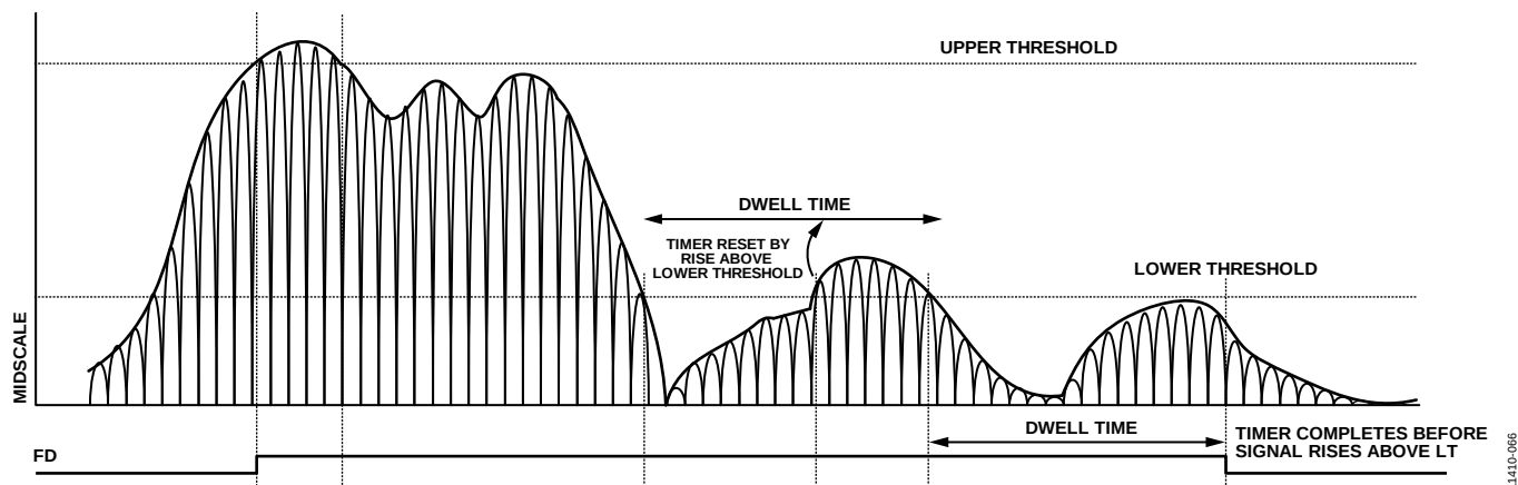
Figure 66. Threshold Settings for FD Signals
