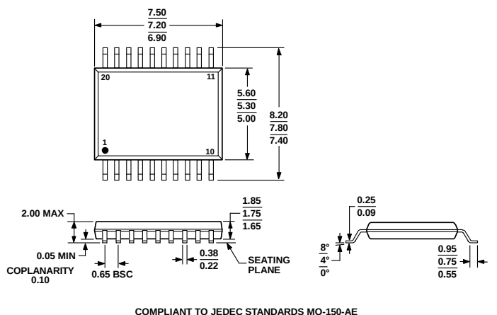
Figure 22. 20-Lead Shrink Small Outline Package [SSOP] (RS-20)
