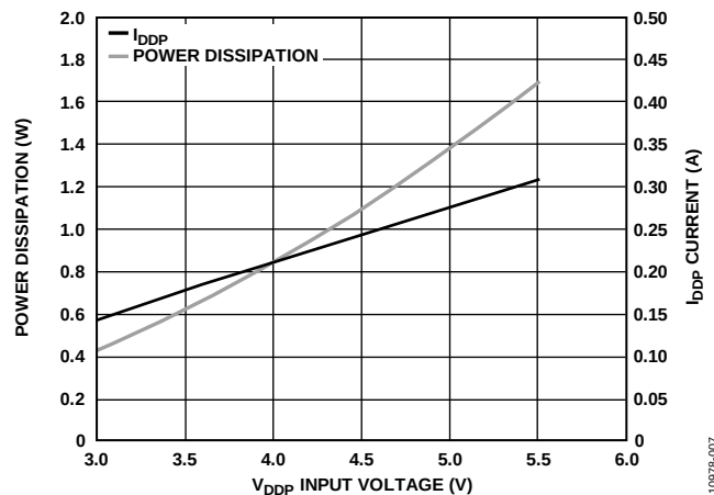
Figure 7. Typical Short-Circuit Input Current and Power vs. V_{DDP} Supply Voltage
