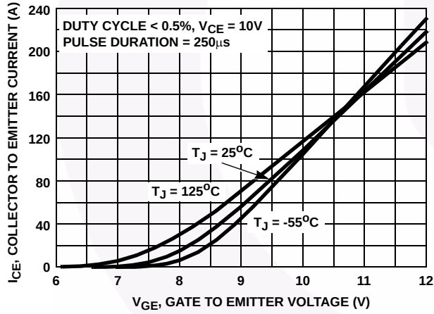
FIGURE 13. TRANSFER CHARACTERISTIC
