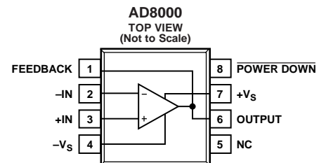
Figure 1. 8-Lead AD8000, 3 mm \times 3 mm LFCSP_VD (CP-8-2)
