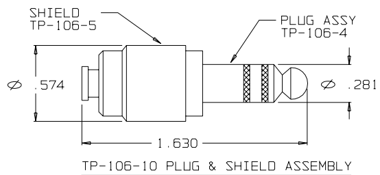
TP-106-10 PLUG & SHIELD ASSEMBLY
