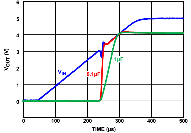
FIGURE 131. TURN-ON TIME
