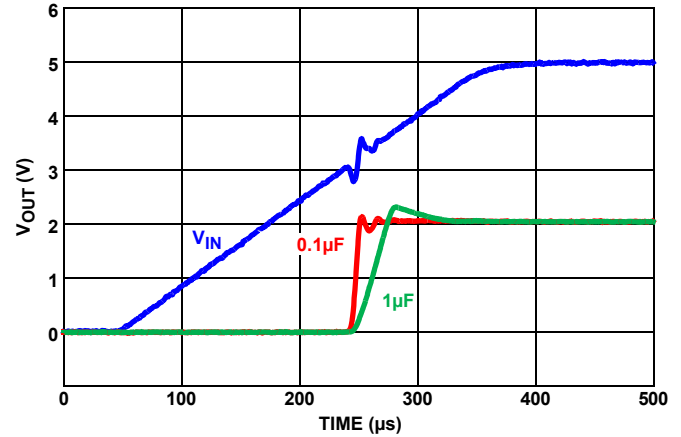
FIGURE 63. TURN-ON TIME
