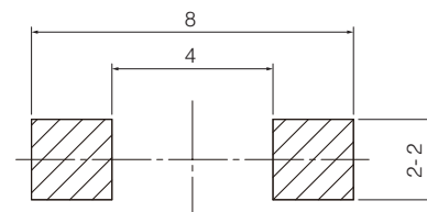
Land pattern plan
