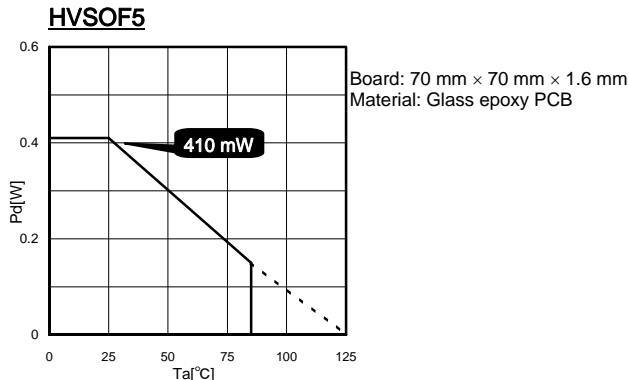
Fig. 26 HVSO5 Power Dissipation/Power Dissipation Reduction (Example)
