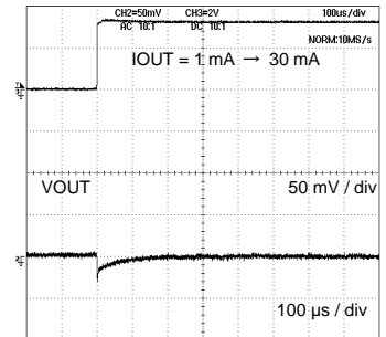
Fig.21 Load Response (Co = 2.2 μF) (BH33NB1WHFV)
