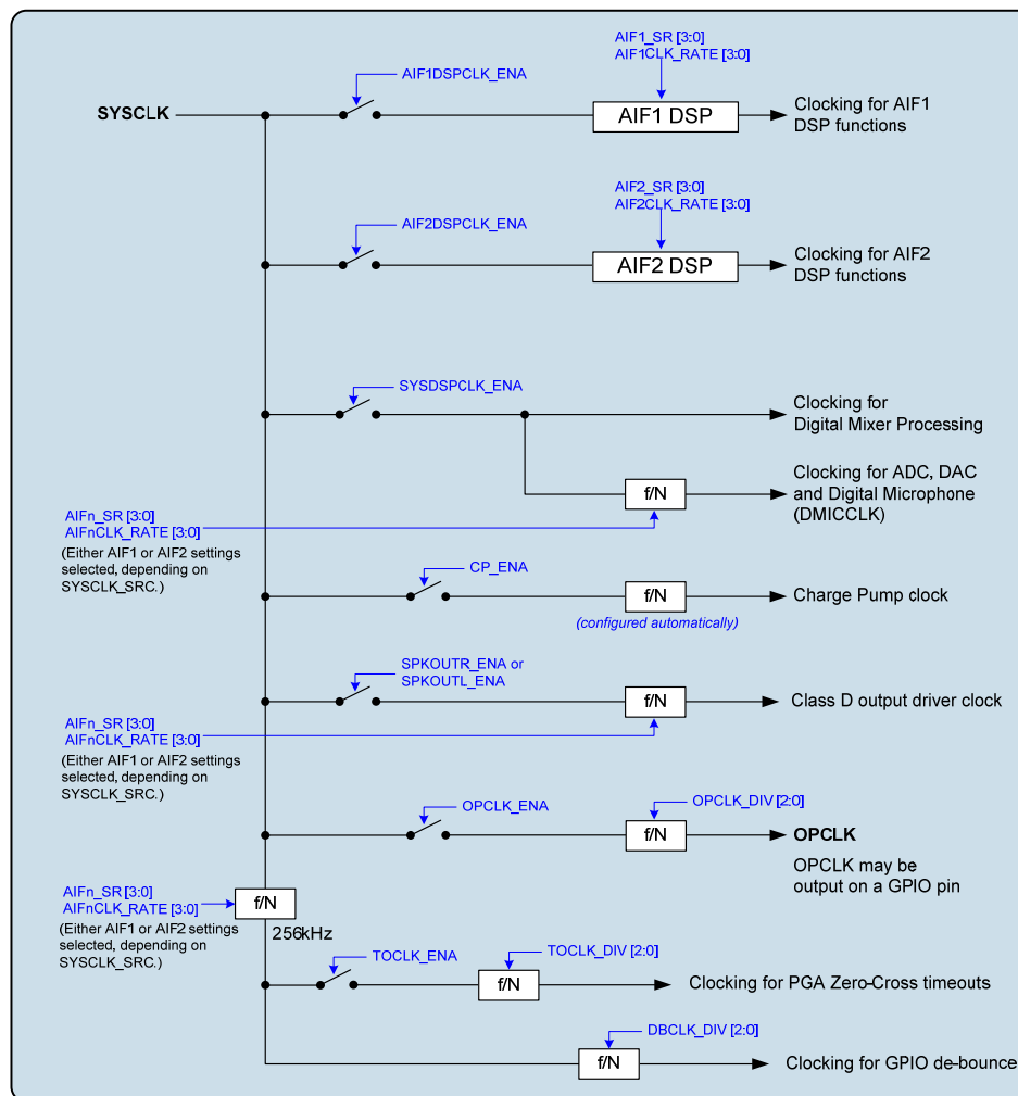
Figure 69 System Clocking
