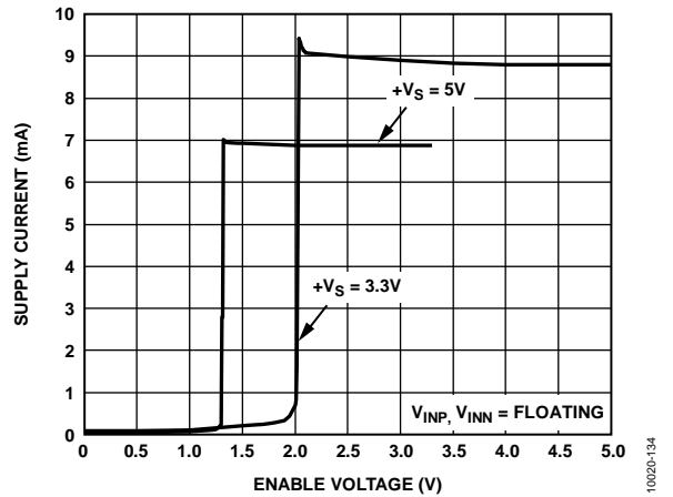
Figure 20. Supply Current vs. Enable Voltage
