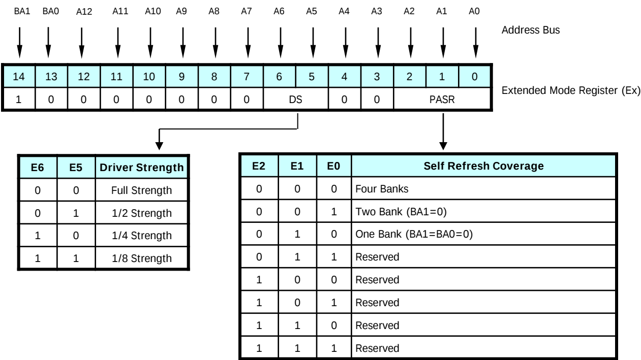
Figure5 : Extended Mode Set (EMRS) Register
