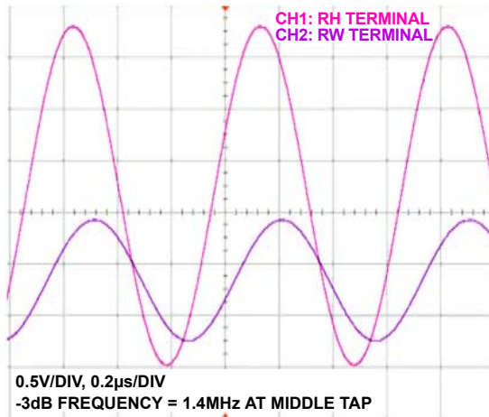
FIGURE 23. 10k \Omega -3dB CUT OFF FREQUENCY
