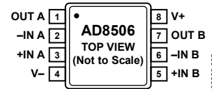
Figure 3. 8-Lead MSOP (RM-8)
