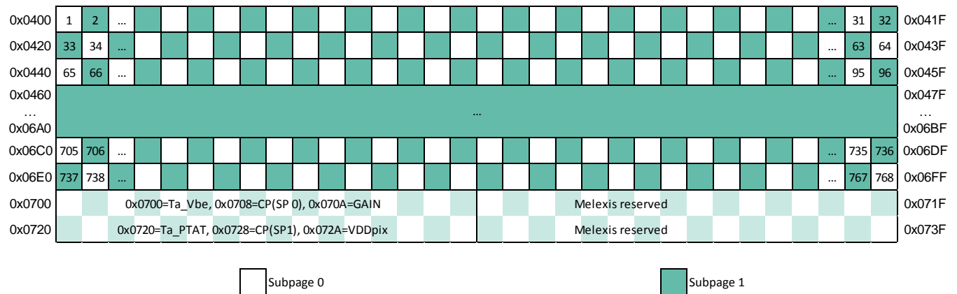
Figure 14 RAM memory map (Chess pattern mode) – factory default mode
