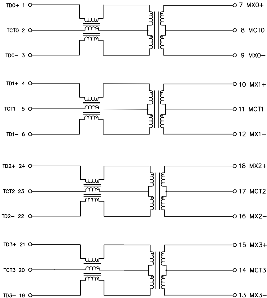
SCHMATIC
