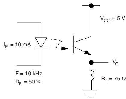
Fig. 10 - Switching Schematic
