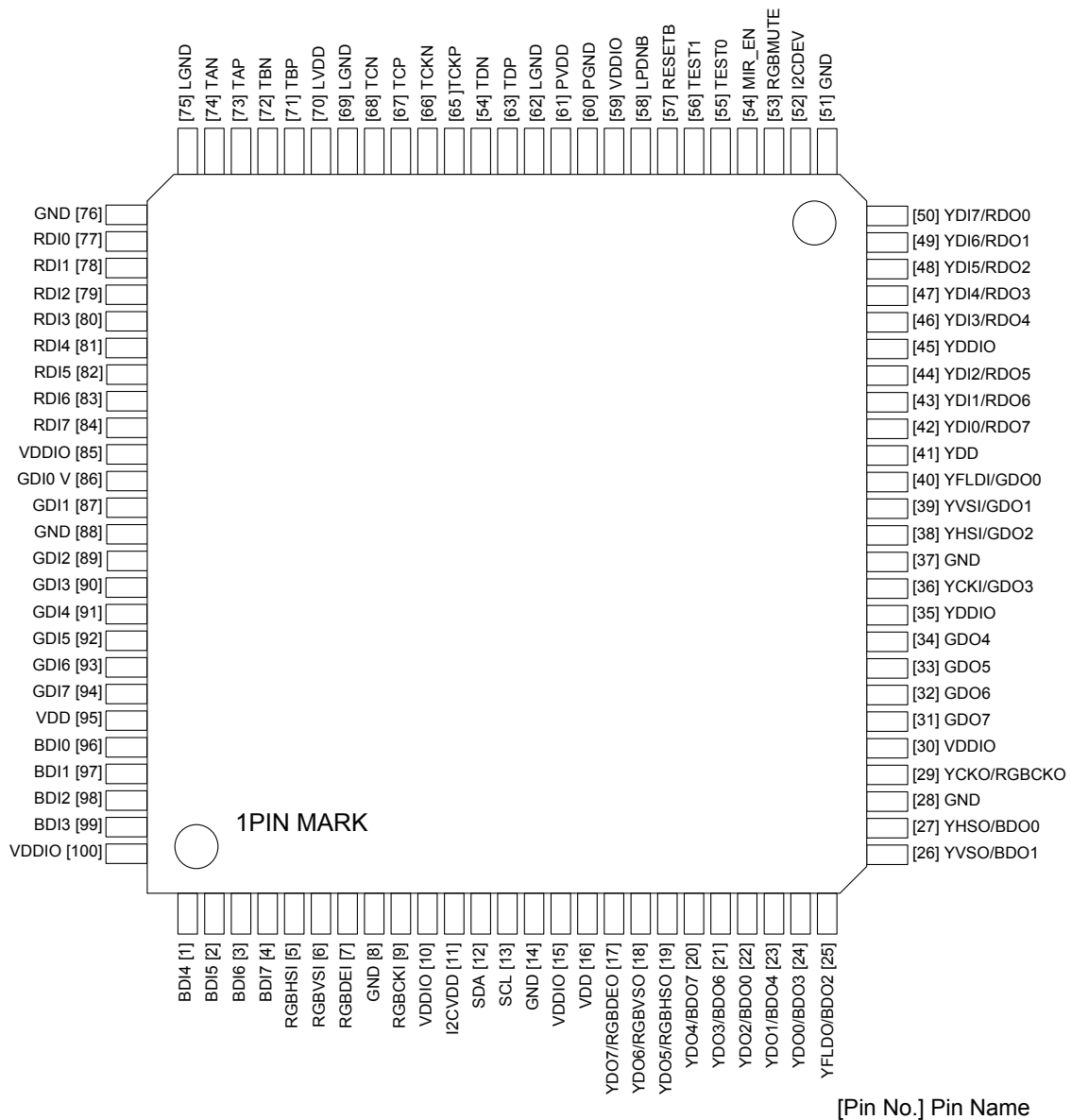
Fig.2 Pin configurations
