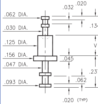
2705-X-00-XX-00-00-07-0 Swage mount in .129 hole
