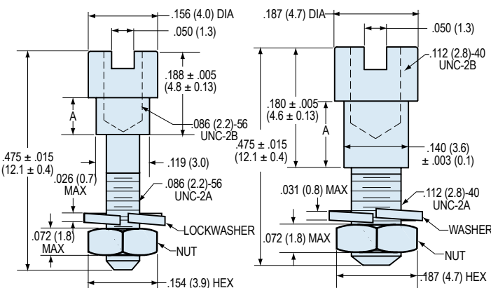
Figure 1 #2-56 Jackpost
