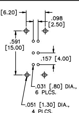
P.C. BOARD LAYOUT
