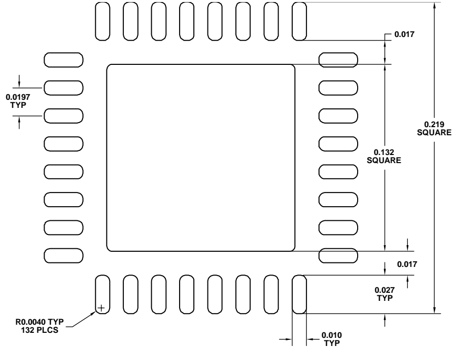
Figure 49. Solder Paste Stencil of the ADMV1010-EVALZ
