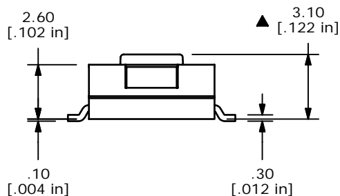
TERMINALS TO BE COLPLANAR WITH IN 0.10mm
