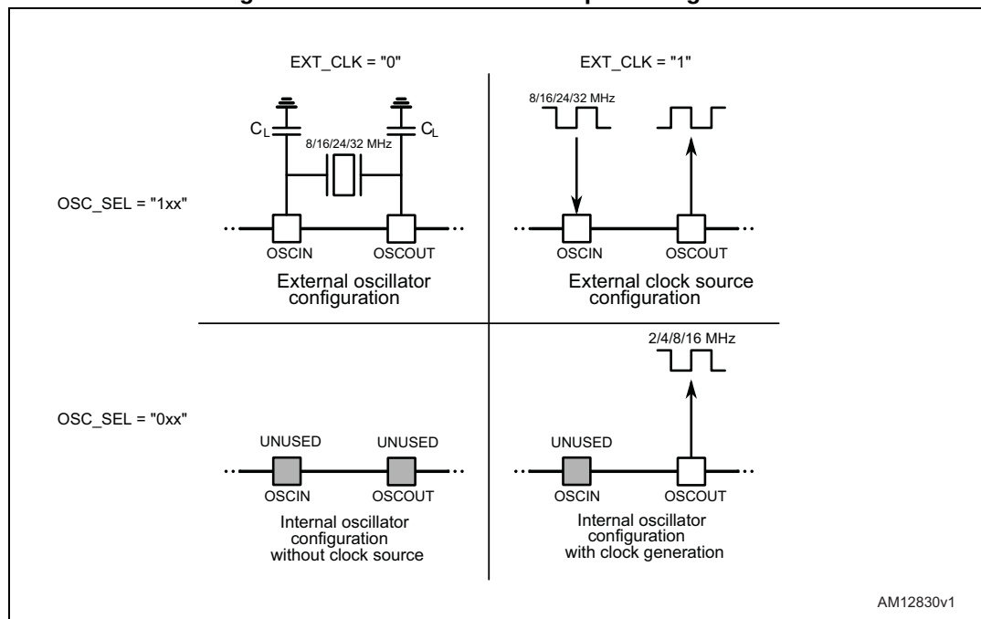
Figure 12. OSCIN and OSCOUT pin configuration
